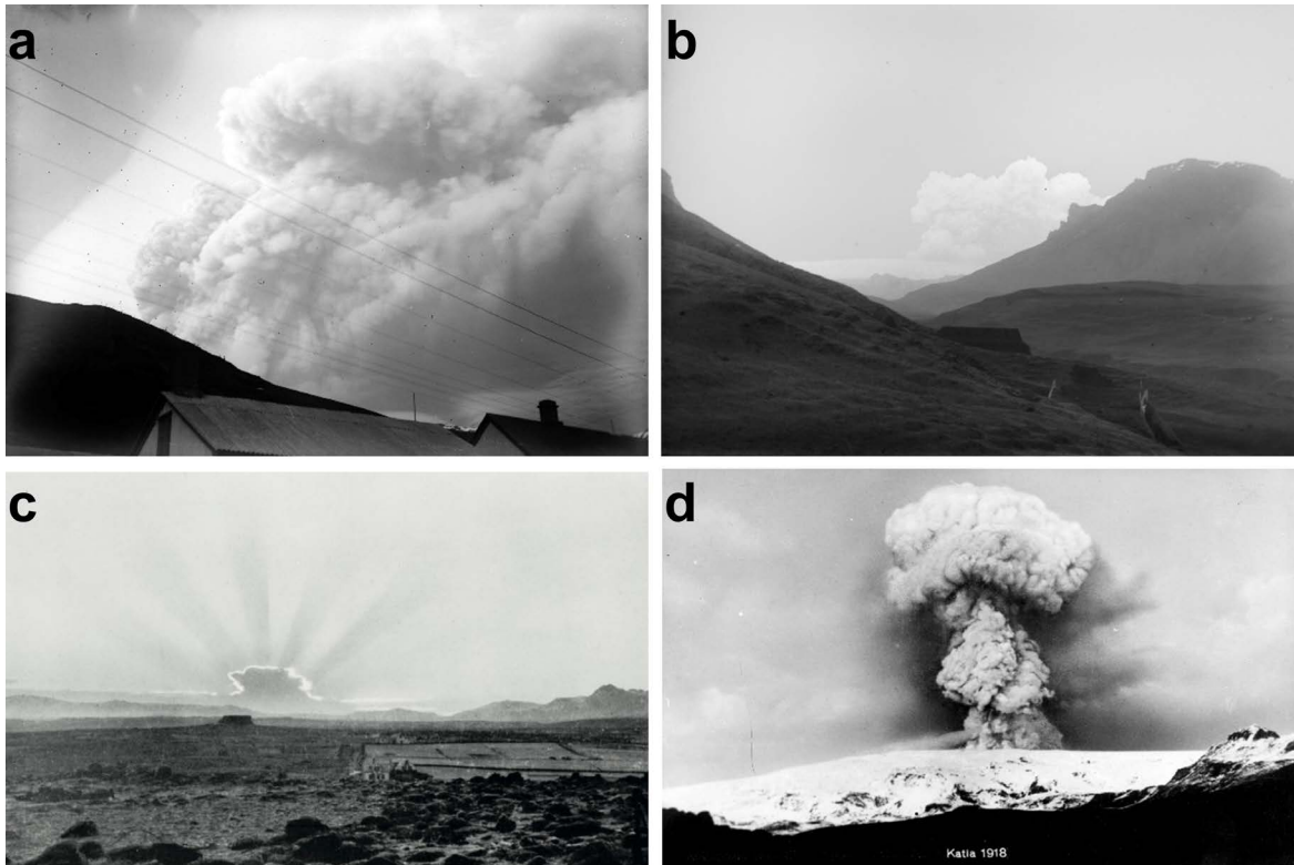
Figure 4. Photos of the Katla 1918 eruption plume. a) This photo is taken from the Vík village, 20 km from the eruption site, with a view towards north. The rim with snow seen between the houses is Hatta, the mountain to the right in (b). The plume apparently rises to about 15 km above sea level (Larsen and Högnadóttir, this issue). The photo is undated, but probably taken on October 12 (Photo: Þorlákur Sverrisson). b) The photo is taken about 1 km north of Vík, most likely on October 20. The plume rises 3–3.5 km above the vents (4–4.5 km a.s.l.). (Photo: Þorlákur Sverrisson). c) The 1918 eruption plume seen from Reykjavík. The photo is undated, but cannot be from October 12, as it is taken in the early morning (Photo: Magnús Ólafsson). The plume was seen from Reykjavík on October 15 and 16 (Morgunblaðið, Oct. 16 and 17, 1918) and this photo could be taken on either of these dates. The plume is 7–8 km high (a.s.l.). d) The Katla eruption near its end. The photo was taken about 2.5 km to the north of Vík, on November 2. The plume rises to 7–8 km a.s.l. (Photo: Kjartan Guðmundsson). – Ljósmyndir af gosmekki í Kötlugosinu 1918. a) Ljósmynd Þorláks Sverrissonar, tekin í Vík í Mýrdal, 20 km frá gosstöðvunum, ódagsett en líklega tekin 12. október. Milli húsanna grillir í efstu fjallsbrúinir Höttu. Gosmökkurinn rís um 15 km y.s. (sjá einnig grein Guðrúnar Larsen og Þórdísar Högnadóttur í þessu hefti). b) Ljósmynd Þorláks Sverrissonar tekin um 1 km norðan við Vík, ódagsett en líklega tekin 20. október. Mökkurinn rís 3–3,5 km yfir gosstöðvarnar (4–4,5 km y.s). c) Gosmökkurinn séður úr Reykjavík, ljósmynd Magnúsar Ólafssonar, ódagsett en tekin að morgni til og er því ekki frá 12. október. Gosmökkurinn er 7–8 km hár (y.s). Hann sást frá Reykjavík 15. og 16. október (Morgunblaðið, 16. og 17. október 1918). d) Kötlugosið undir lokin. Ljósmynd Kjartans Guðmundssonar tekin 2. nóvember 1918. Gosmökkurinn rís 7–8 km y.s.
