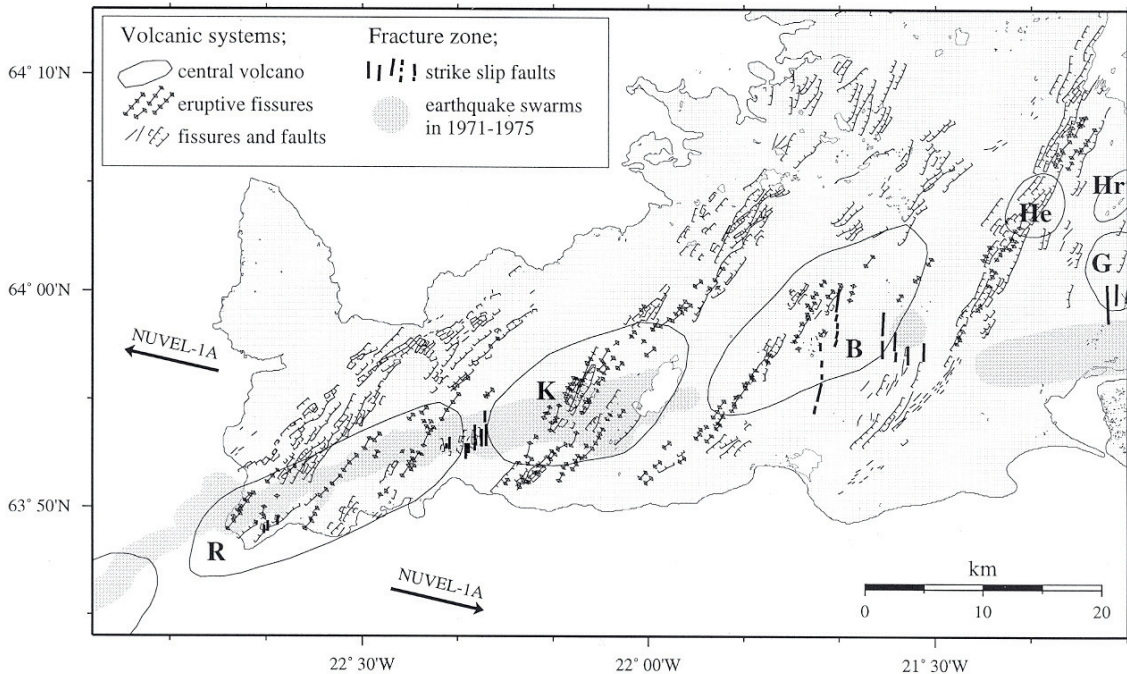
Figure 4. Faults and fissures on the Reykjanes Peninsula, modified from Hreinsdóttir et al. (2001) and Clifton and Kattenhorn (2007). – Misgengi og sprungur á Reykjaneskaga.
