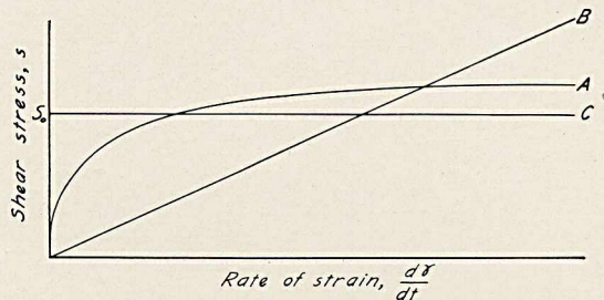
Fig.1. Stress-strain relation for fluids and plastic bodies.
