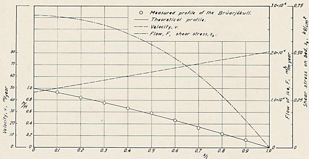
Figure 2. Section through Brúarjökull, a glacier in the northern Vatnajökull in Iceland. This is approximately a central section with H = 600 m and L = 20 km. The velocity v and flow F are theoretical values from equations (21) and (22).
